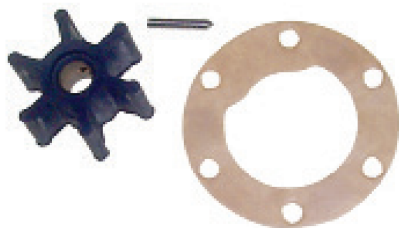
18-3079 IMPELLER KIT Replaces: 875807-0, 3586498 Johnson Pump 09-806B Sherwood 9979K 6 FINS Neoprene Jabsco 4528-0001 Side Width \frac{3}{4} " Dia. 1 \frac{9}{16} "
