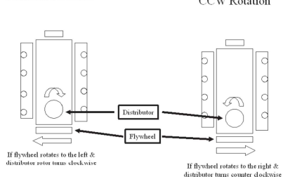
Standard Rotation
