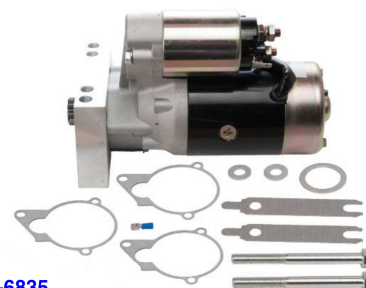
18-6835 STARTER Replaces: GM Engines Universal Used on all GM Engines with either 14 1/4" or 12 3/4" flywheels
