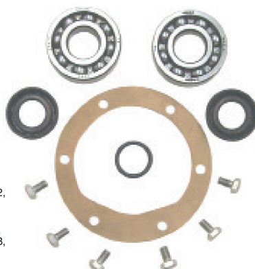
18-3209 WATER PUMP REPAIR KIT Replaces: 875383 AQ165A, 170A, B, C, MD21A (S/N MD103387 & UP), MD21B
