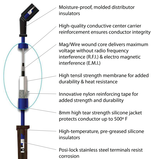
OMC MARINE IGNITION WIRES APPLICATION
