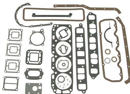
18-4374 OVERHAUL GASKET SET For: 140 HP and 3.0L (1973-88)
