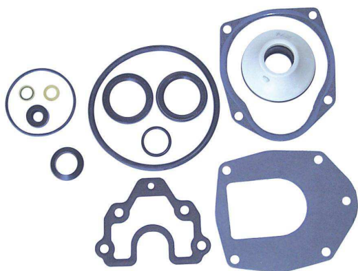
18-2725 LOWER UNIT SEAL KIT Replaces: 26-830749A01
