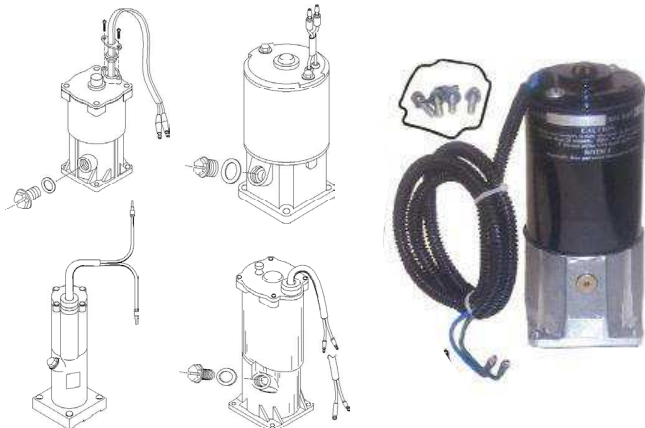
18-6777 TILT/TRIM MOTOR Replaces: 818903A1, 819762A4-A7, 819479A1, 819480A1, 81977A8-A9, 822870A1, 830250A3-T3, 832021A1-T4-A2-T2, 855654A1-T2, 19217A1-A5, 854472A2, A3, A4 Contains: All parts necessary, a new 2-wire motor/reservoir, drive shaft coupler, oil seal, O-ring and hardware. Yellow fill plug. Square base O-ring.
