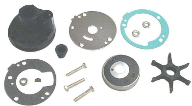
18-3426 WATER PUMP KIT With Housing Replaces: 42431M, 84829M, 97793M, 97793T
