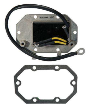
18-5832 REGULATOR/RECTIFIER Replaces: 583266, 583689, 586000, 584424
