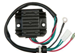
18-6651 VOLTAGE REGULATOR Replaces: 66V-81960-00-00 Fits: GP1200 (2000-02); XL, XLT1200 (1999-05)
