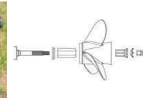
Fig. 8 The forward thrust washer MUST be installed first. Failure to install a forward thrust washer will cause gearcase damage and potential injury.
